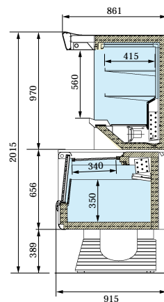
AKRON SELF 140/200 TB-TN
